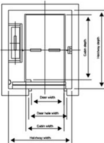
Hoistway plan
