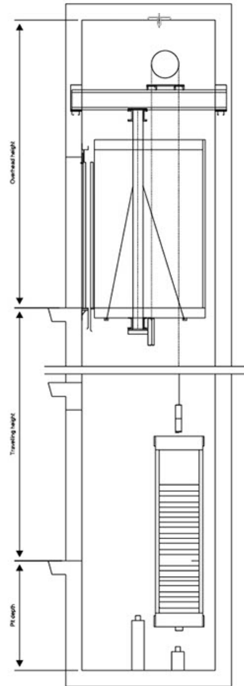
Hoistway elevator
