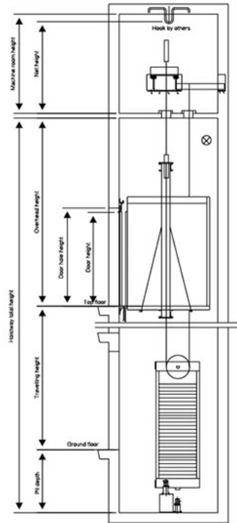
Hoistway elevator
