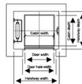
Hoistway plan
