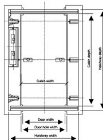
Hoistway plan
