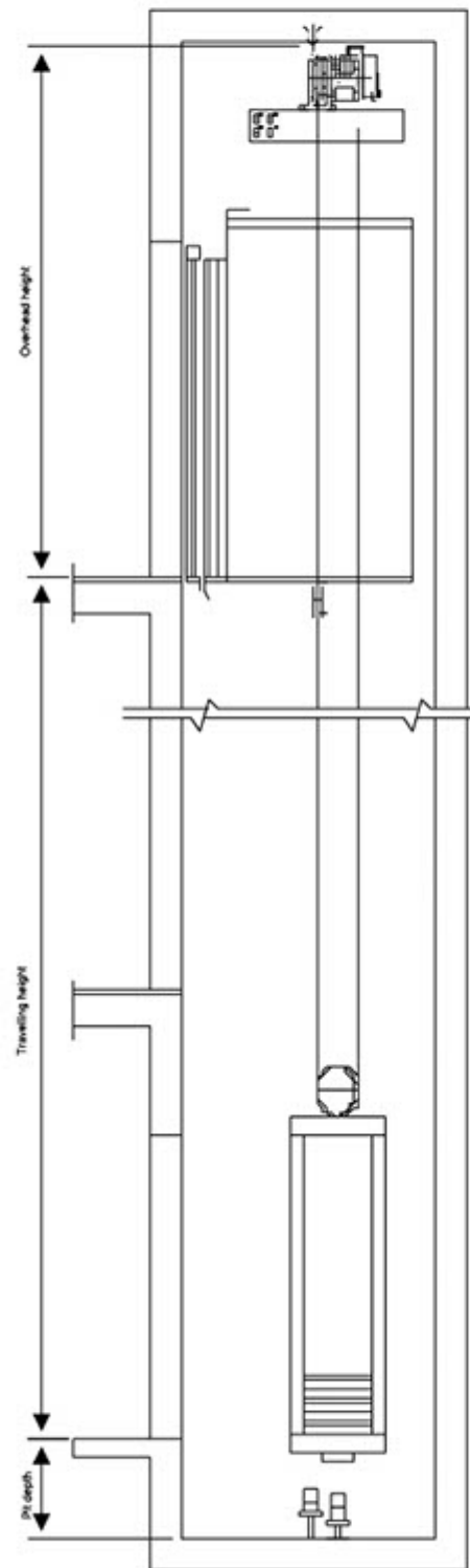
Hoistway elevator
